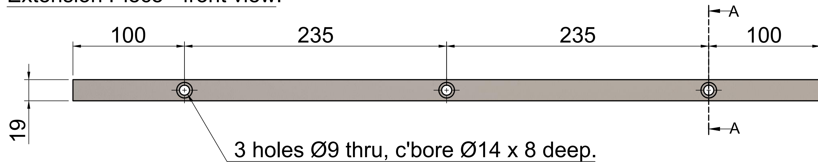
Extension Piece - front view:
