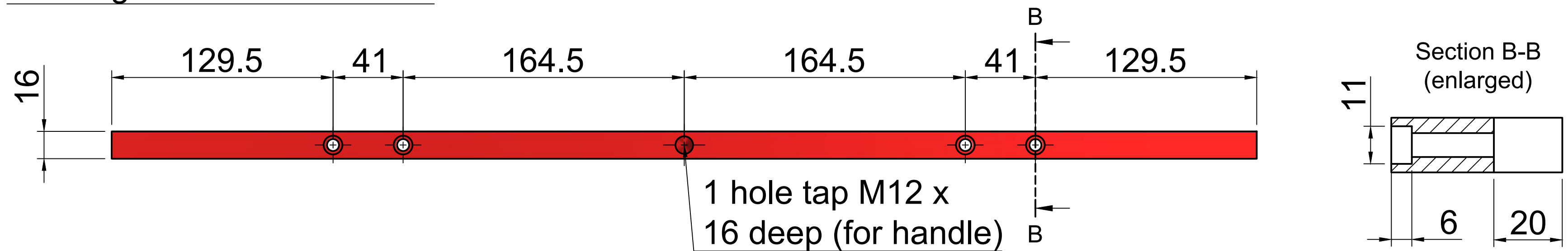
Extension Piece - front view:
