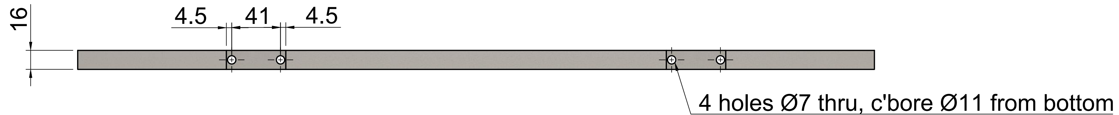
Bending Beam - bottom view:
